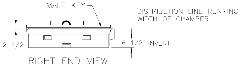
SECTION VIEW
