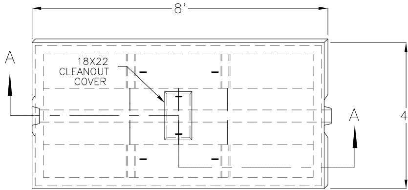
PLAN VIEW
