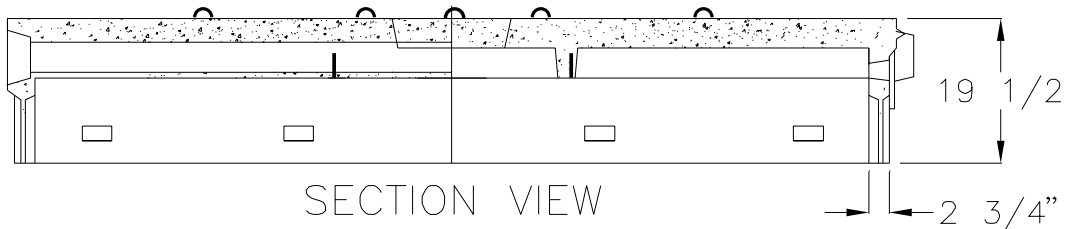
SIDE VIEW
